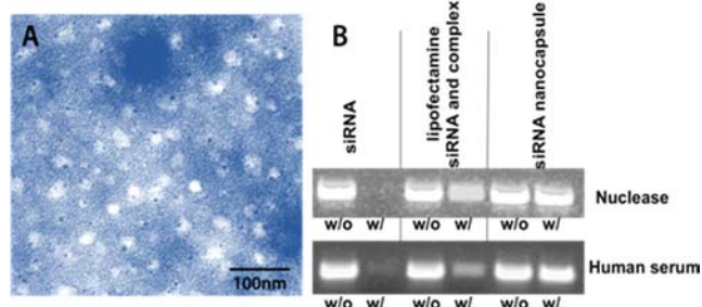
Figure 1. (A) TEM image of siRNA nanocapsules; (B) sensitivity of siRNA to nuclease and human serum. siRNA complexed with lipofectamine and siRNA nanocapsules were incubated for 1 h with nuclease (up) and human serum (down), respectively. Then, siRNAs were extracted from lipofectamine and nanocapsules with chloroform/0.1% SDS–0.5 M NaCl. Samples were run on 4% agarose gel and imaged with ImageQuant LAS4000.
